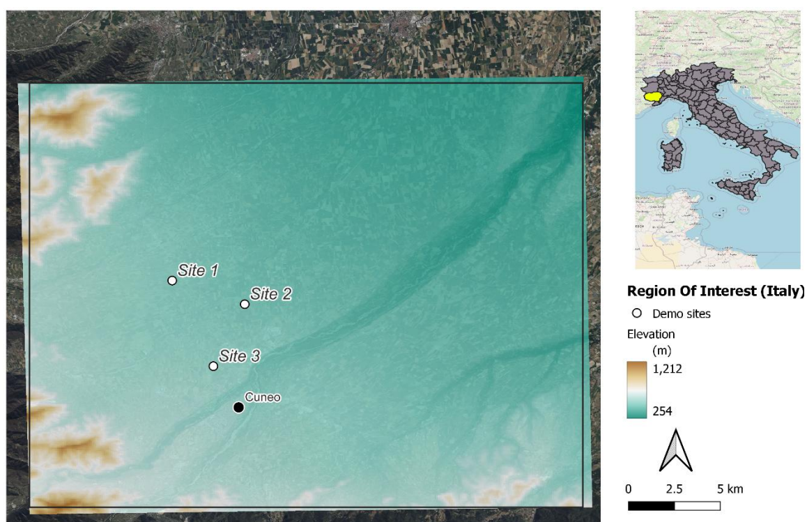
Figure 11. DEM of the pilot area in Piedmont, Italy, one of the three areas within the MAGDA project.
