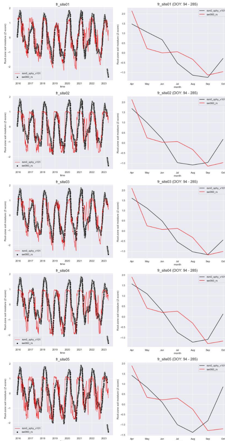
Figure 29. Left: Seasonality plots with daily normalized soil moisture values, Right: Seasonality plots with interannual monthly average soil moisture values for France
