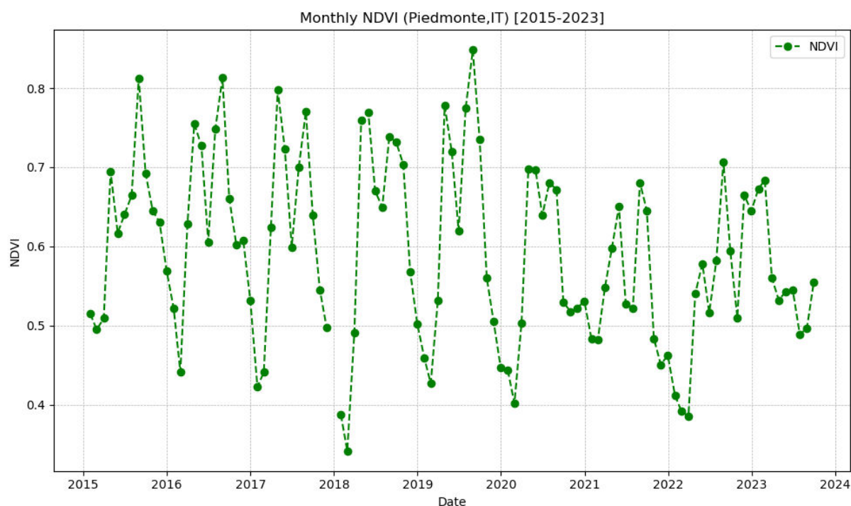
Figure 15. Monthly Mean NDVI in one of the demo sites in Piedmont, Italy.
