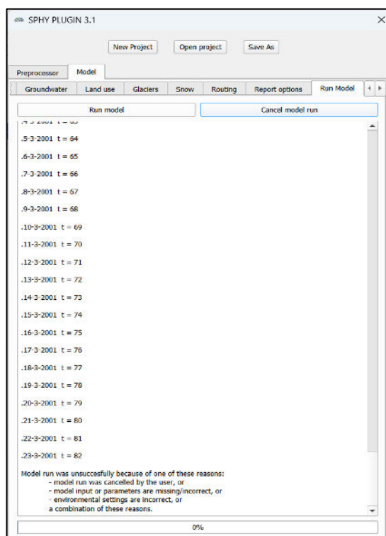
Figure 53. Example log screen output of cancelled model run.
