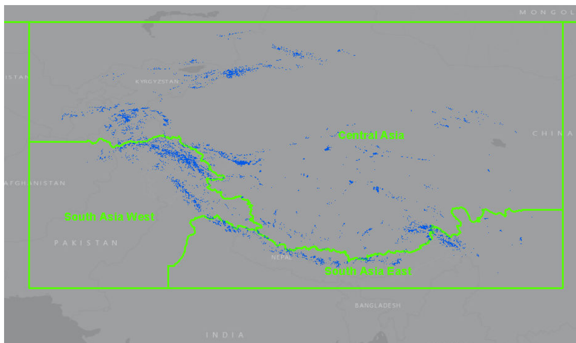
Randolph Glacier Inventory glacier outlines (blue) included in Hindu Kush-Himalaya database. RGI regions are indicated by green polygons.
